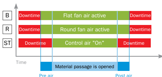
Illustration of pre- and post air delay with SATAjet ROB spray guns
